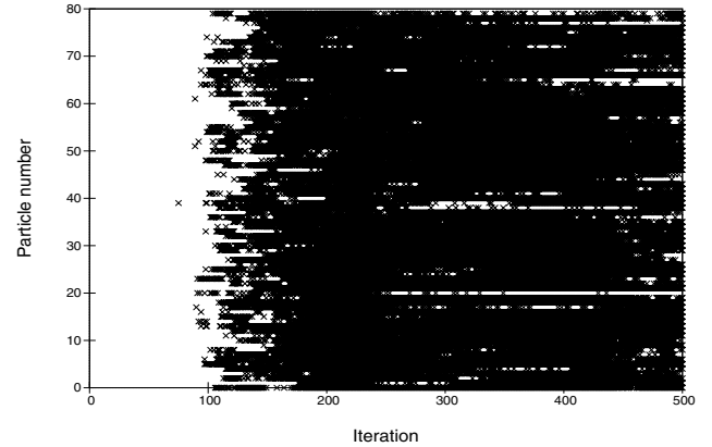
Fig. 1. Stagnation of particles in Tribe-PSO
